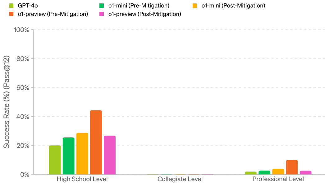
Success Rate on Capture-The-Flag (CTF) Challenges
