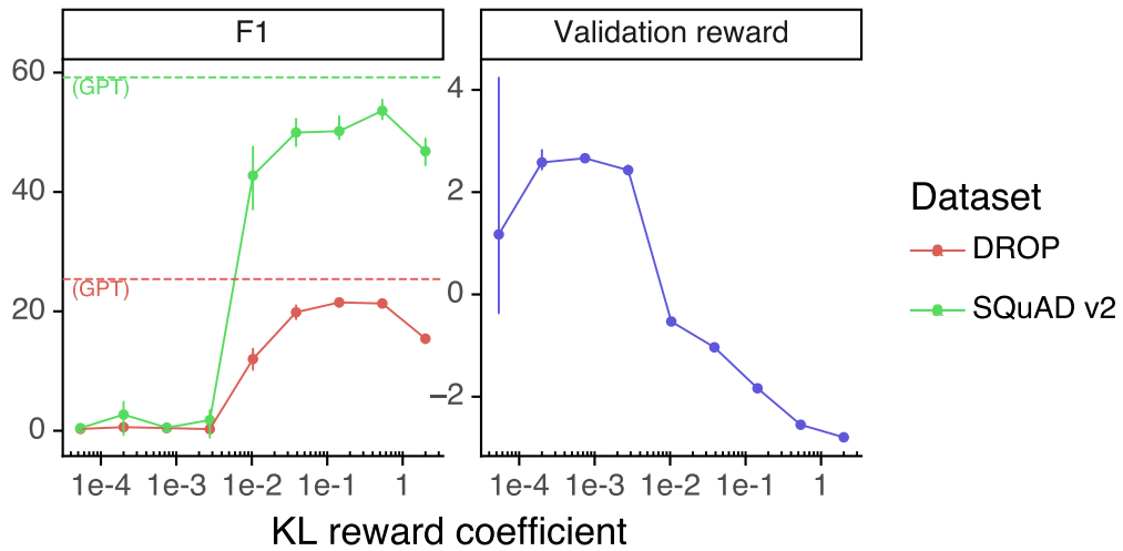
Figure 34: Evaluation on public NLP datasets as a function of KL reward coefficient. Increasing the KL coefficient does not fully mitigate the regressions on DROPP and SQuAD.
