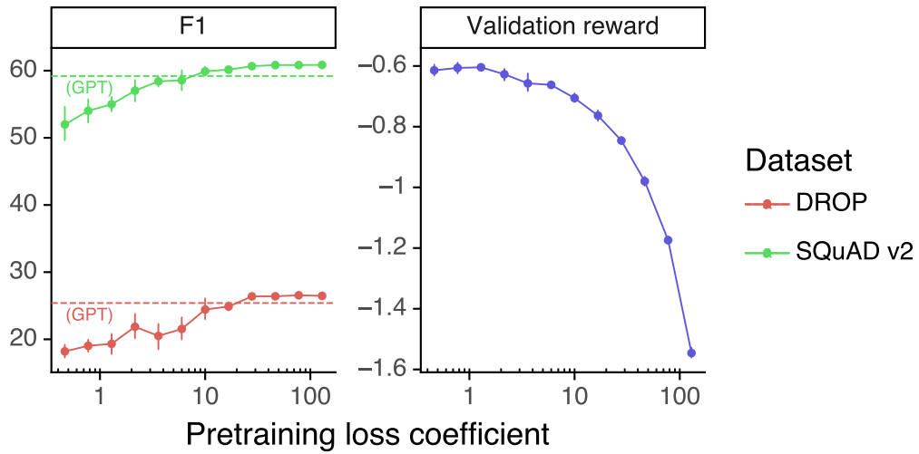
Figure 33: Evaluation on public NLP datasets as a function of pretraining loss coefficient. There is a pretraining coefficient that leads to a significant improvement on DROPP and SQuAD and not much regression on validation reward.
